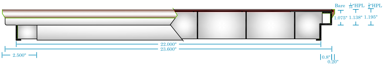
CEI Model GG712 HPL06Z2ST61B (1/16" HPL Finish) and GG712 HPL12Z2ST61B (1/8" HPL Finish) Perforated Air Flow Panel
